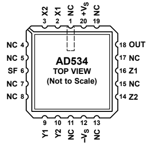
Figure 6. LCC (E-20-1) Pin Configuration
