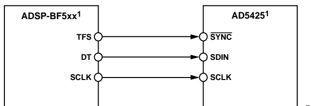
Figure 40. ADSP-BF504 to ADSP-BF592 Device Family to AD5425 Interface (ADSP-BFxx Denotes the ADSP-BF504 to ADSP-BF592)
