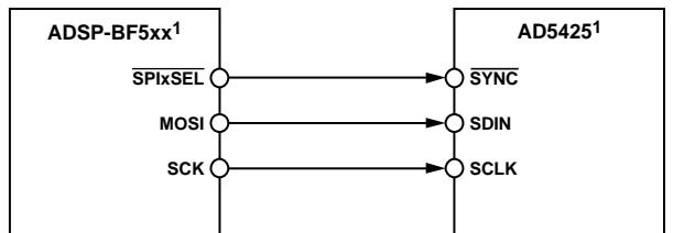
Figure 39. ADSP-BF504 to ADSP-BF592 Device Family to AD5425 Interface (ADSP-BFxx Denotes the ADSP-BF504 to ADSP-BF592)
