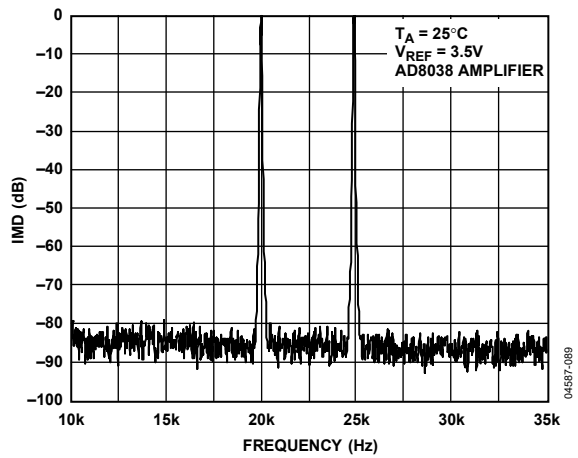
Figure 40. Narrow-Band IMD, f_{OUT} = 20 kHz, 25 kHz, Clock = 1 MHz
