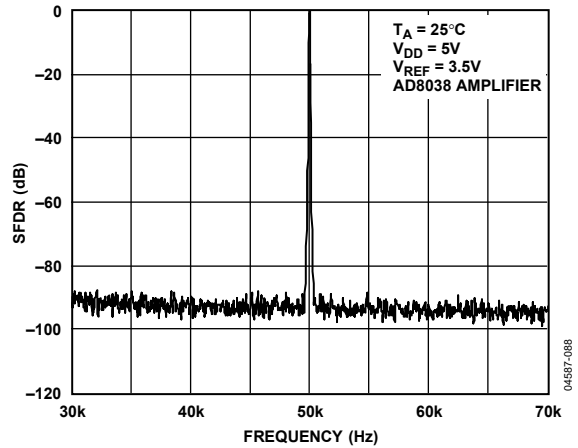
Figure 39. Narrow-Band SFDR, f_{OUT} = 50 kHz, Clock = 1 MHz
