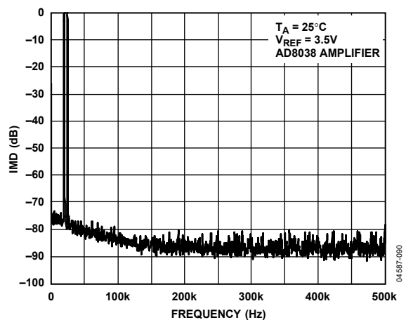
Figure 41. Wideband IMD, f_{OUT} = 20 kHz, 25 kHz, Clock = 1 MHz
