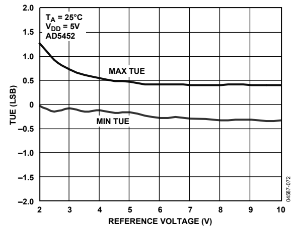
Figure 20. TUE vs. Reference Voltage
