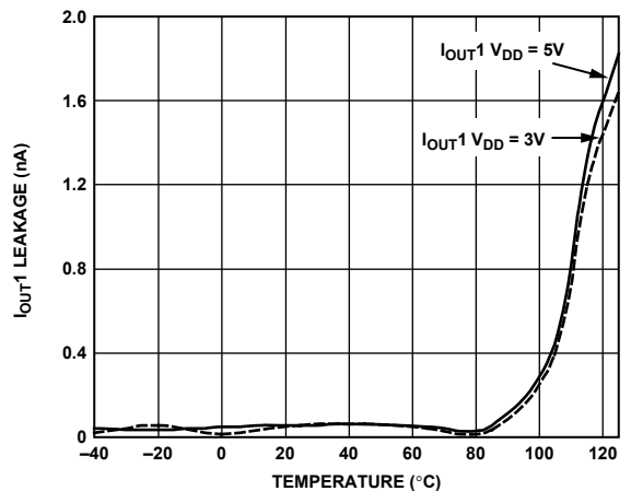
Figure 23. IOUT1 Leakage Current vs. Temperature
