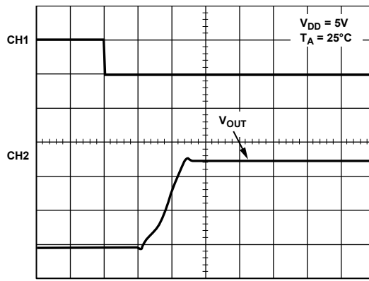
CH1 5V, CH2 1V, TIME BASE = 2 \mu s/DIV
