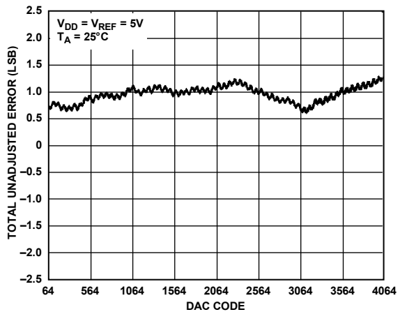
Figure 8. AD5621 Total Unadjusted Error (TUE)
