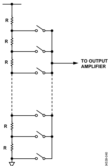
Figure 40. Resistor String
