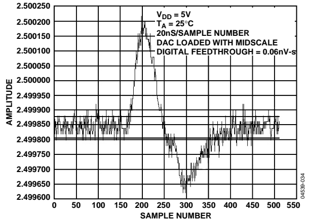
Figure 34. Digital Feedthrough
