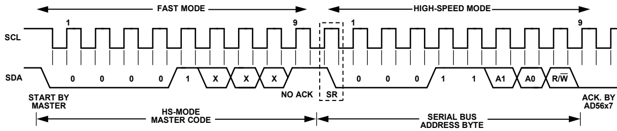
Figure 56. Placing the AD5627RBMZ-2/AD5667RBMZ-2 in High Speed Mode
