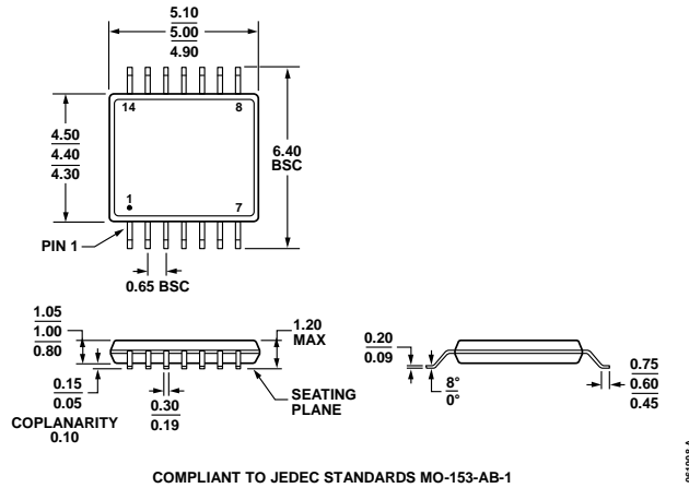
Figure 62. 14-Lead Thin Shrink Small Outline Package [TSSOP] (RU-14) Dimensions shown in millimeters
