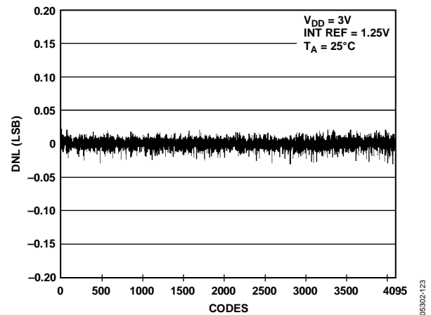
Figure 24. DNL AD5628-1
