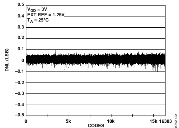
Figure 23. DNL AD5648-1
