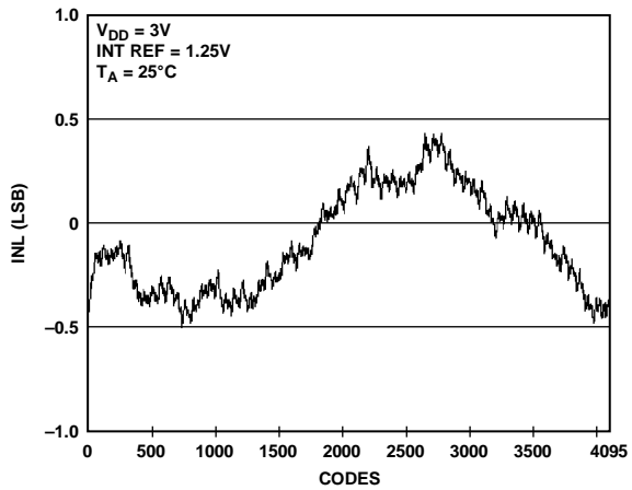
Figure 21. INL AD5628-1
