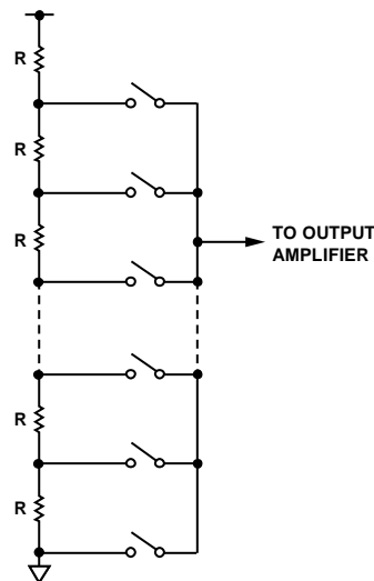
Figure 56. Resistor String
