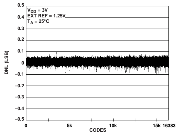
Figure 23. DNL AD5648-1
