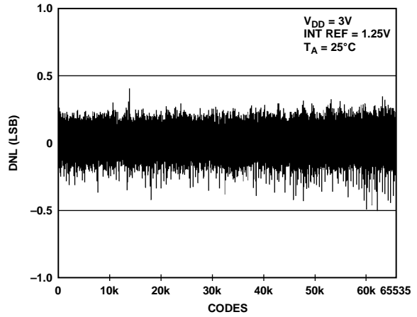
Figure 22. DNL AD5668-1
