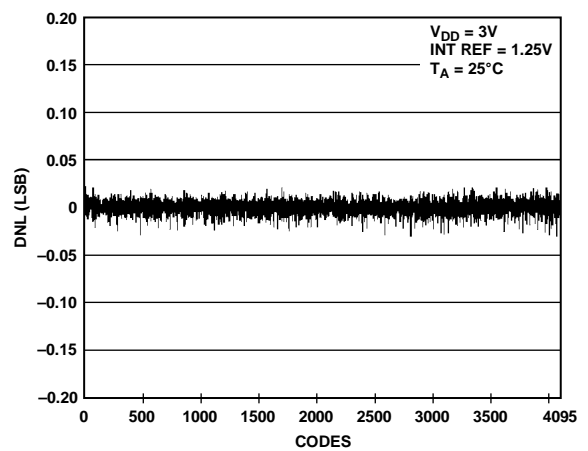
Figure 24. DNL AD5628-1
