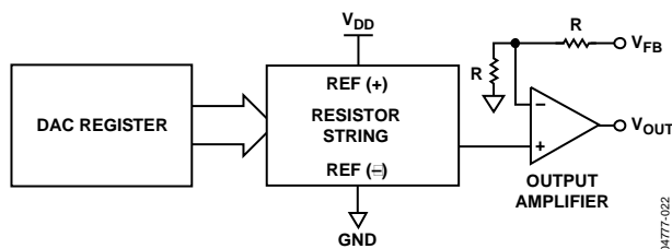
Figure 39. DAC Architecture
