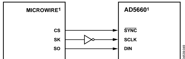
Figure 49. AD5660-to-MICROWIRE Interface
