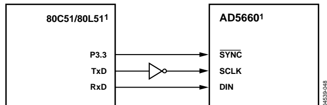
Figure 48. AD5660-to-80C51/80L51 Interface
