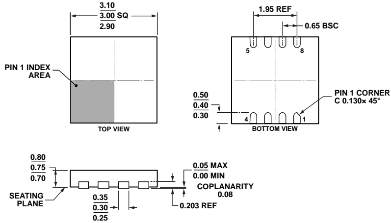
COMPLIANT TO JEDEC STANDARDS MO-229-WEEC-2 Figure 56. 8-Lead Lead Frame Chip Scale Package [LFCSL_WD] 3 mm x 3 mm Body, Very Very Thin, Dual Lead (CP-8-15) Dimensions shown in millimeters
