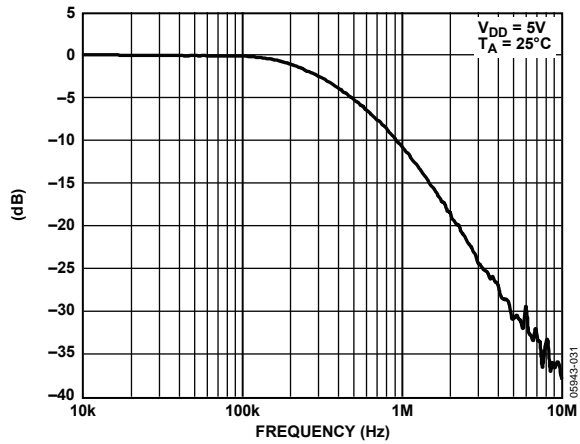
Figure 29. Multiplying Bandwidth
