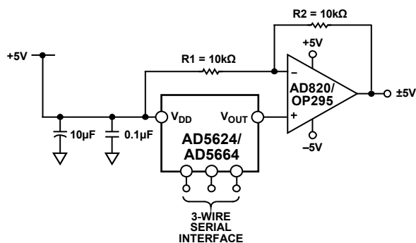
Figure 41. Bipolar Operation with the AD5624/AD5664
