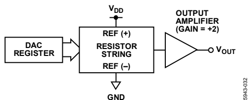
Figure 30. DAC Architecture
