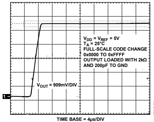
Figure 20. Full-Scale Settling Time, 5V
