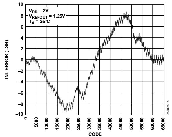
Figure 9. INL—16-Bit DAC, 1.25 V Internal Reference
