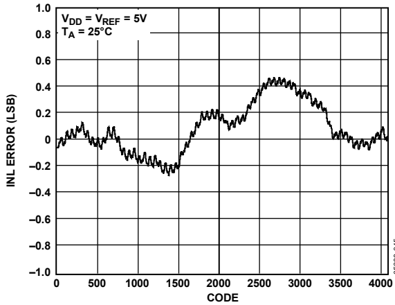
Figure 11. INL—12-Bit DAC
