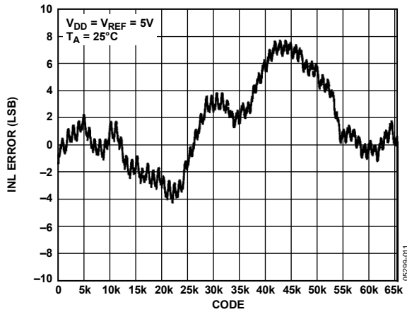
Figure 5. INL—16-Bit DAC
