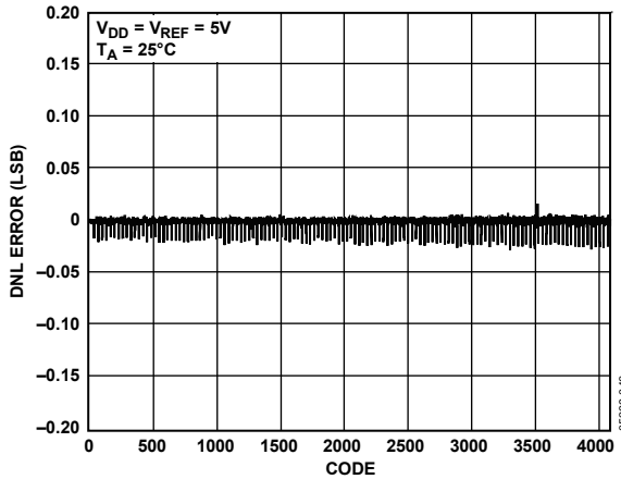
Figure 12. DNL—12-Bit DAC
