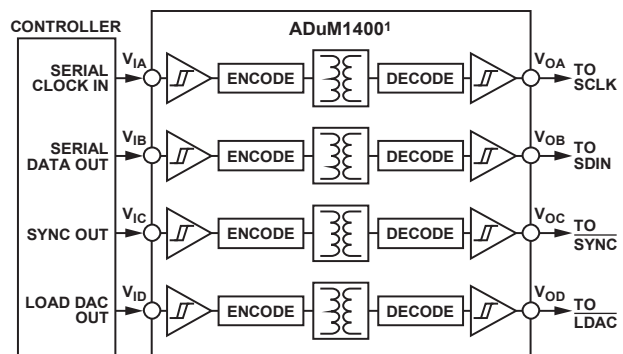
Figure 54. Isolated Interface
