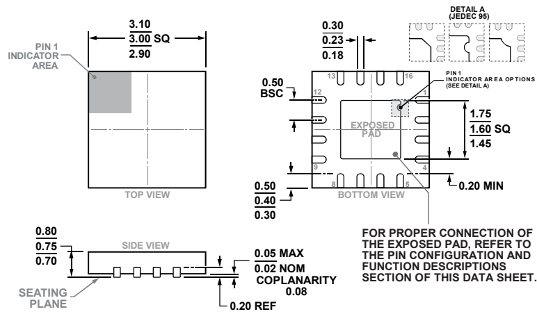
Figure 55. 16-Lead Lead Frame Chip Scale Package [LFCSP_WQ] 3 mm x 3 mm Body, Very Very Thin Quad (CP-16-22)
