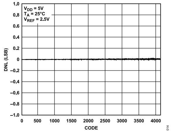
Figure 14. AD5691R DNL
