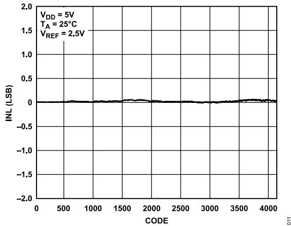
Figure 11. AD5691R INL
