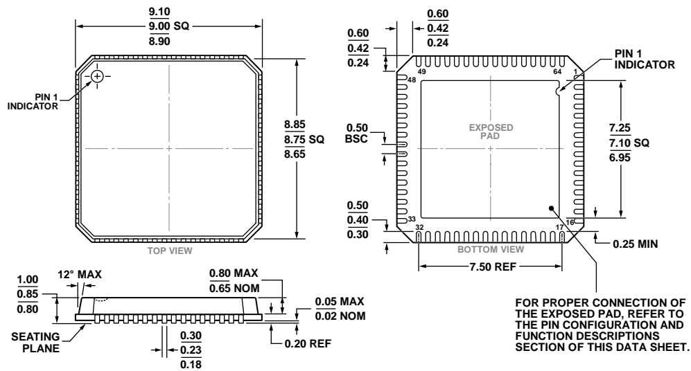
Figure 68. 64-Lead Lead Frame Chip Scale Package [LFCSP_VQ]
