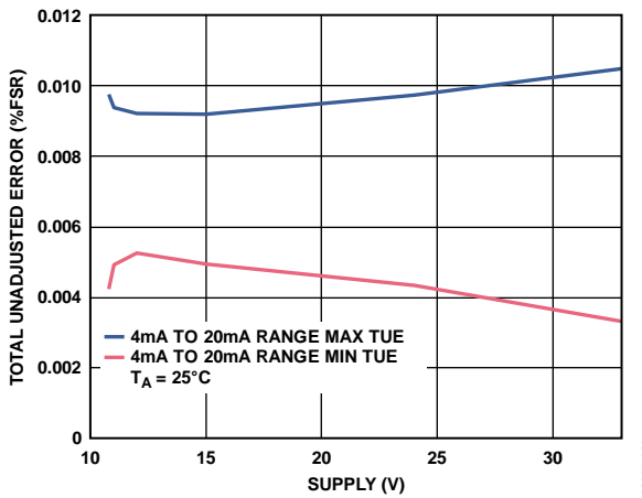
Figure 22. Total Unadjusted Error vs. AV_{DD} , External R_{SET}
