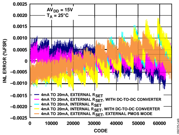
Figure 9. Integral Nonlinearity vs. Code
