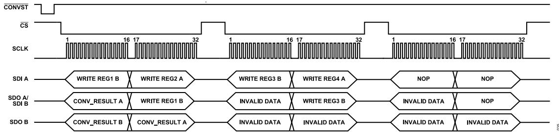
Figure 62. Multiple Register Write in a Two-Target Daisy-Chain Mode Configuration
