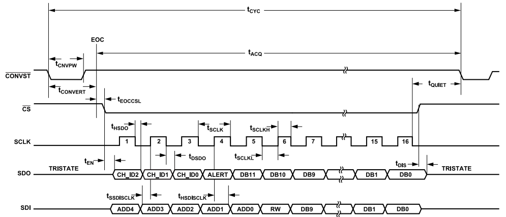
Figure 4. Serial Port Timing
