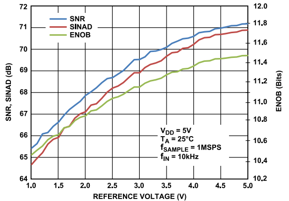
Figure 19. SNR, SINAD, and ENOB vs. Reference Voltage
