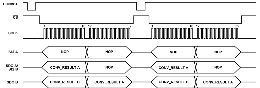
Figure 58. Conversion in a Two-Target Daisy-Chain Mode Configuration
