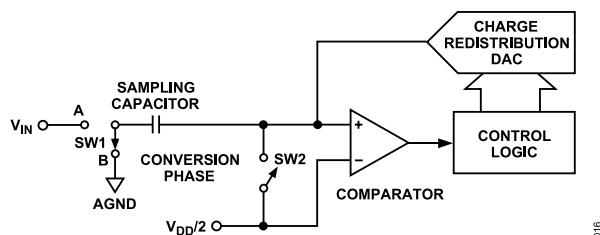
Figure 41. ADC Conversion Phase
