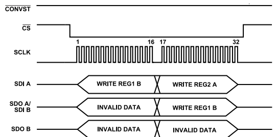
Figure 59. Single Register Write in a Two-Target Daisy-Chain Mode Configuration
