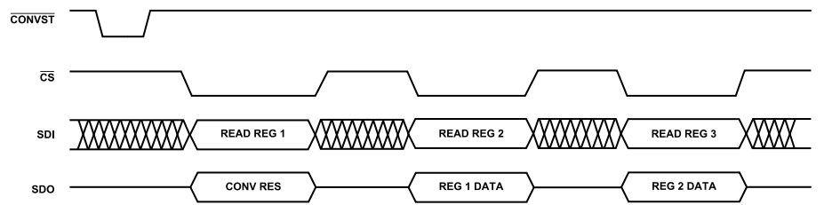
Figure 52. Serial Interface Register Read
