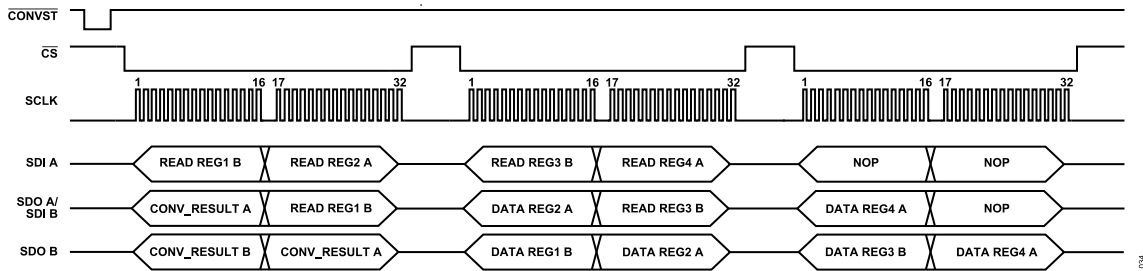
Figure 61. Multiple Register Read in a Two-Target Daisy-Chain Mode Configuration
