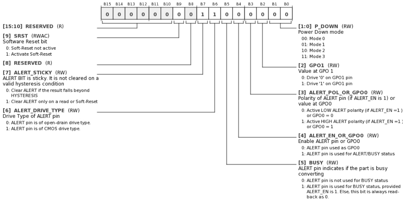
Figure 49. Configuration Register
