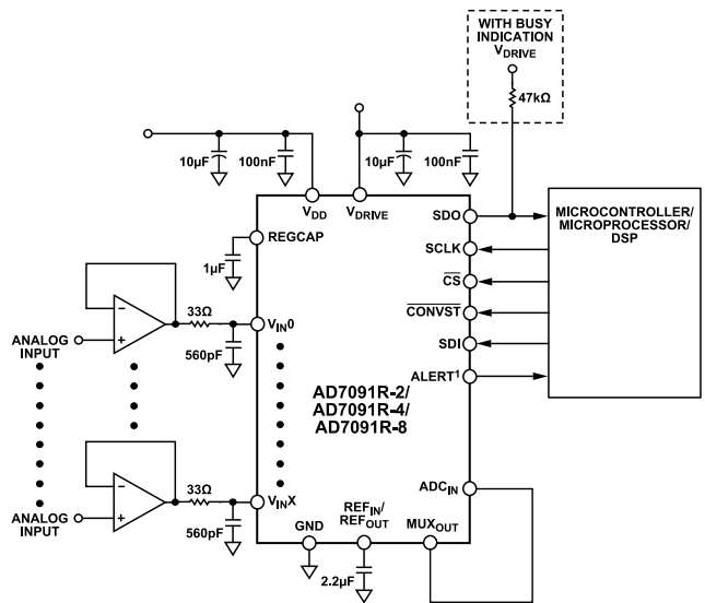
Figure 46. Typical Connection Diagram Without Optional Buffer
