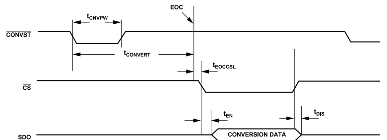
Figure 54. Serial Interface Read Timing in Normal Mode
