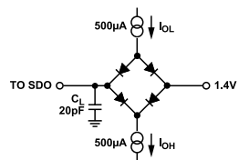
Figure 2. Load Circuit for Digital Interface Timing
