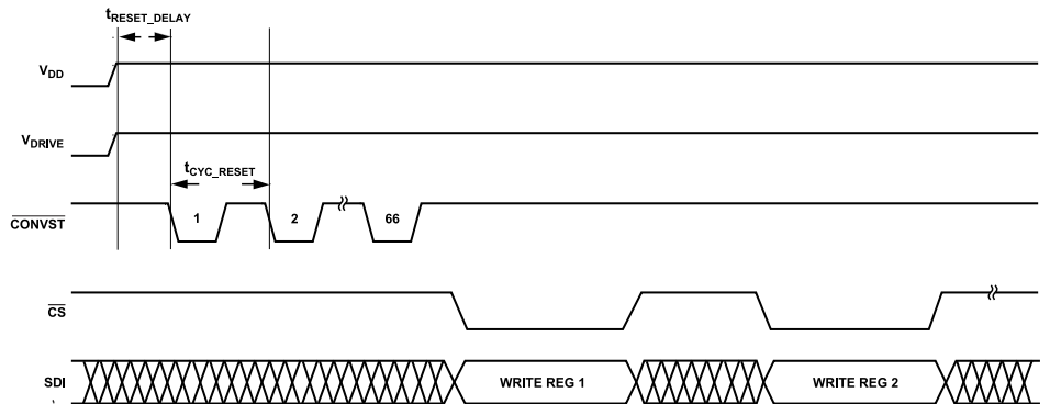
Figure 53. Power On Software Reset Timing
