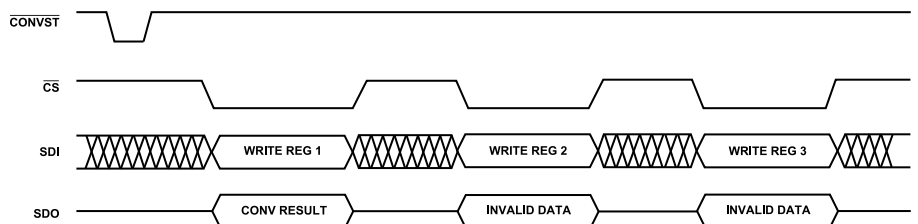
Figure 51. Serial Interface Register Write
