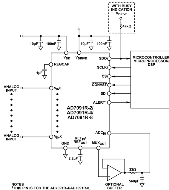
Figure 45. Typical Connection Diagram with Optional Buffer
