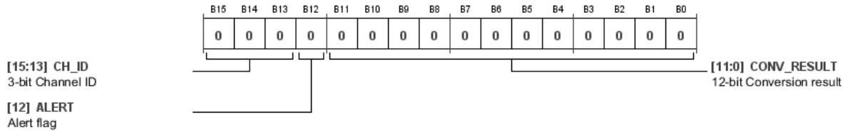
Figure 47. Conversion Result Register
