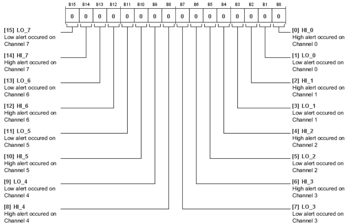
Figure 50. Alert Indication Register (Figure Shows Default Register Value of 0, Indicating No Alert Has Occurred)
