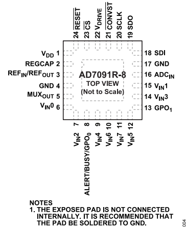
Figure 10. 8-Channel, 24-Lead LFCSP Pin Configuration
