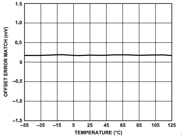
Figure 31. Offset Error Match vs. Temperature
