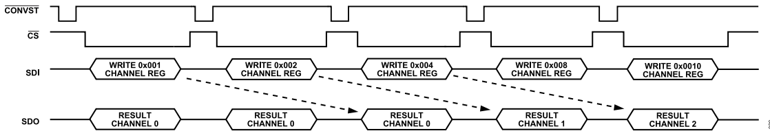
Figure 56. Channel Sequencer Multiple Channel Write
