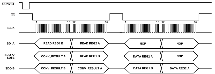
Figure 60. Single Register Read in a Two-Target Daisy-Chain Mode Configuration
