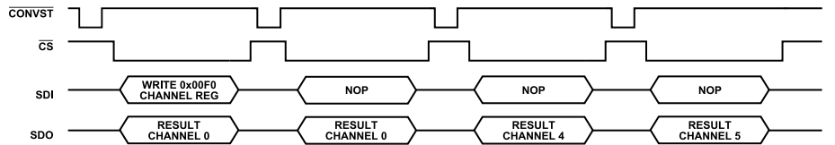
Figure 55. Channel Sequencer
