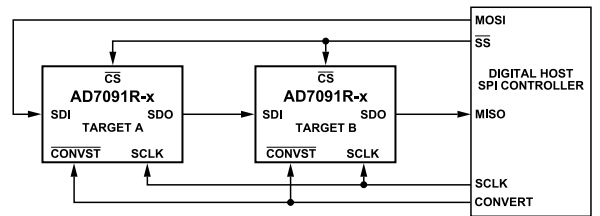
Figure 57. Daisy-Chain Configuration
