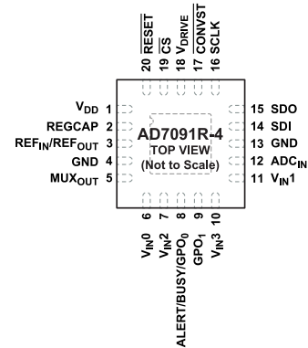
Figure 8. 4-Channel, 20-Lead LFCSP Pin Configuration
