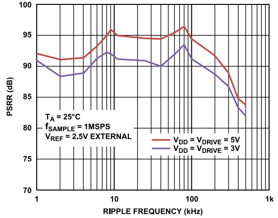
Figure 32. PSRR vs. Ripple Frequency
