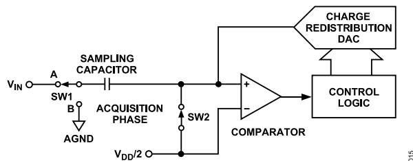
Figure 40. ADC Acquisition Phase
