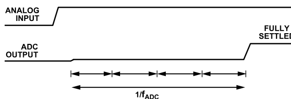
Figure 85. Sinc 4 Zero Latency Operation
