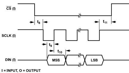
Figure 5. Write Cycle Timing Diagram
