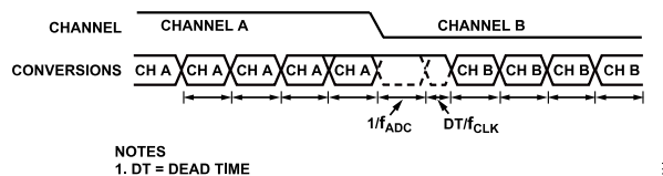
Figure 105. Fast Settling, Sinc 3 + Sinc 1 Filter
