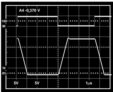
Figure 10. RS-232 Driver; R_L = 5 k\Omega , C_L = 50 pF
