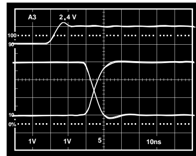
Figure 13. RS-422 Driver; R_{LDIFF} = 100 \Omega , C_{L1} = C_{L2} = 100 pF
