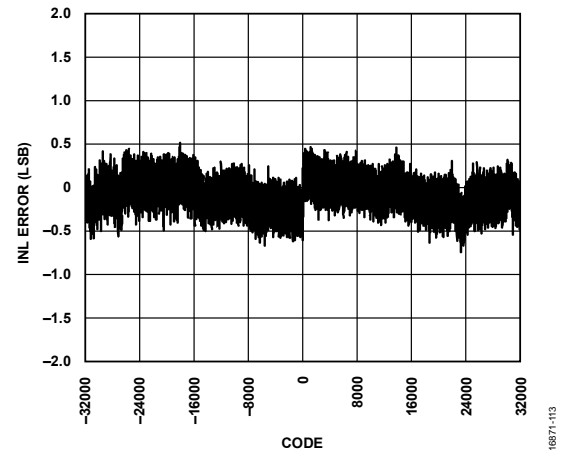
Figure 13. Typical INL Error
