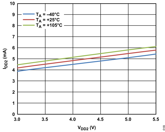
Figure 18. I DD2 vs. V DD2 at Various Temperatures
