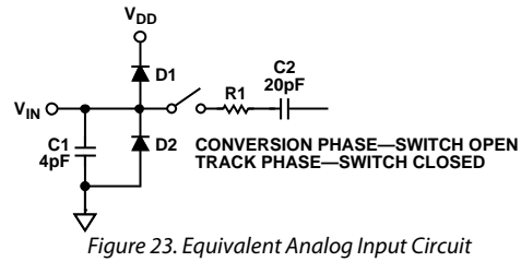
Figure 23. Equivalent Analog Input Circuit
