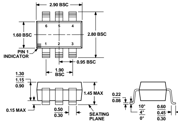
Figure 30. 6-Lead Small Outline Transistor Package [SOT-23] (RJ-6)
