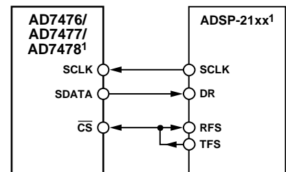
Figure 27. Interfacing to the ADSP-21xx
