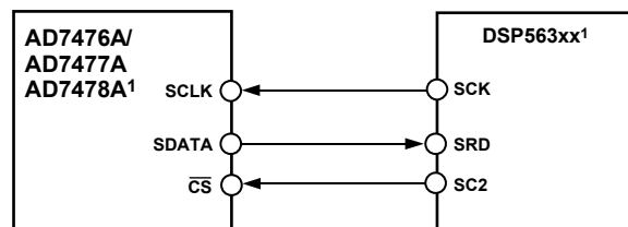
Figure 29. Interfacing to the DSP563xx
