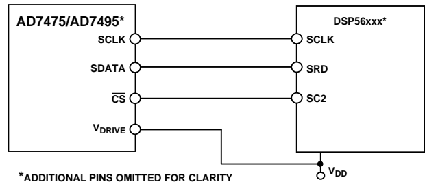
Figure 30. Interfacing to the DSP56xxx
