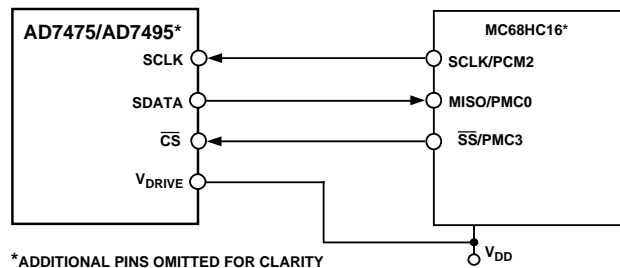
Figure 31. Interfacing to the MC68HC16
