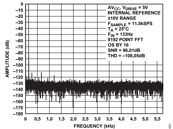
Figure 13. FFT Plot Oversampling By 16, ±10 V Range
