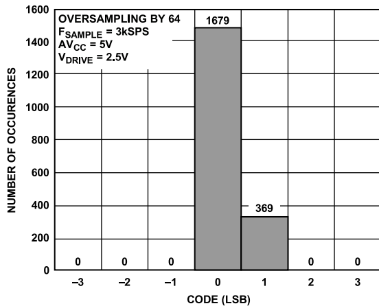
Figure 55. Histogram of Codes—OS x 64 (Two Codes)
