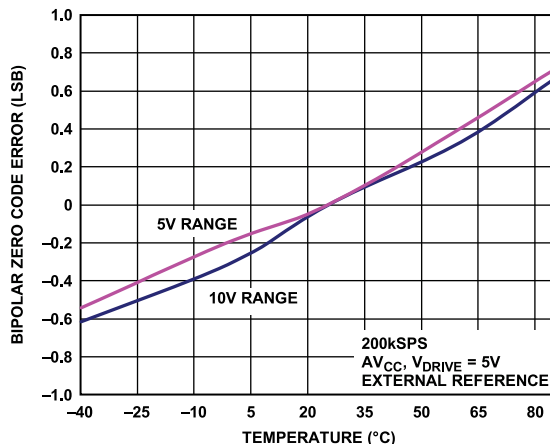
Figure 22. Bipolar Zero Code Error vs. Temperature
