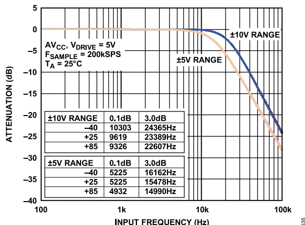
Figure 37. Analog Antialiasing Filter Frequency Response
