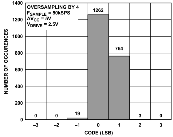
Figure 51. Histogram of Codes—OS x 4 (Four Codes)
