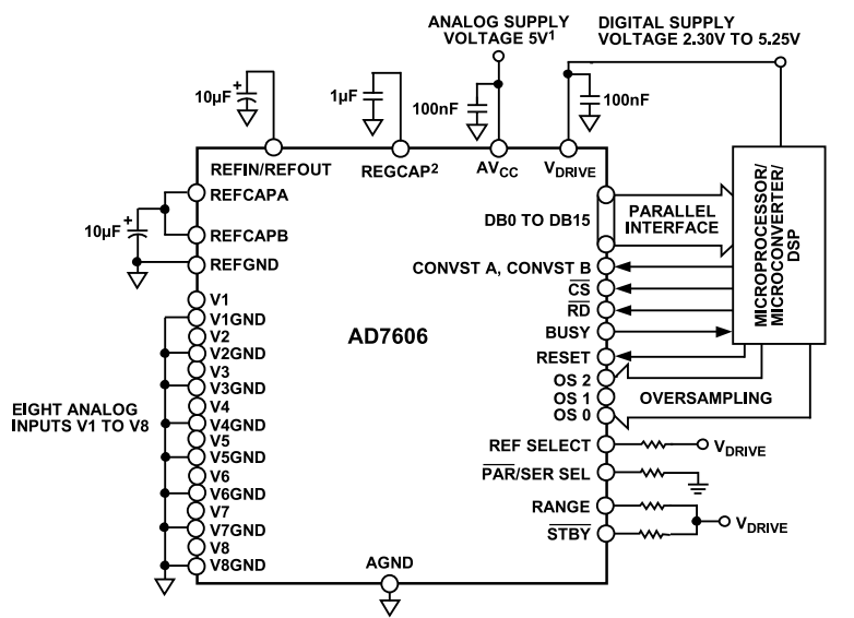
Figure 43. AD7606 Typical Connection Diagram
