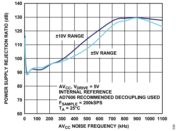
Figure 33. PSRR
