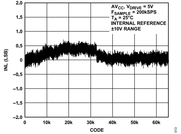
Figure 14. AD7606 Typical INL, ±10 V Range
