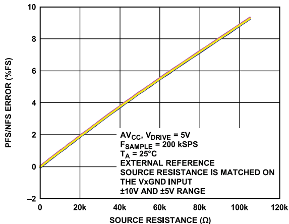
Figure 21. PFS and NFS Error vs. Source Resistance
