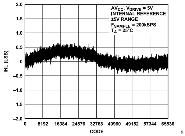
Figure 16. AD7606 Typical INL, ±5 V Range
