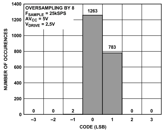
Figure 52. Histogram of Codes—OS x 8 (Three Codes)
