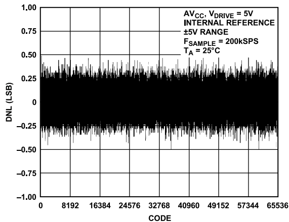
Figure 17. AD7606 Typical DNL, ±5 V Range
