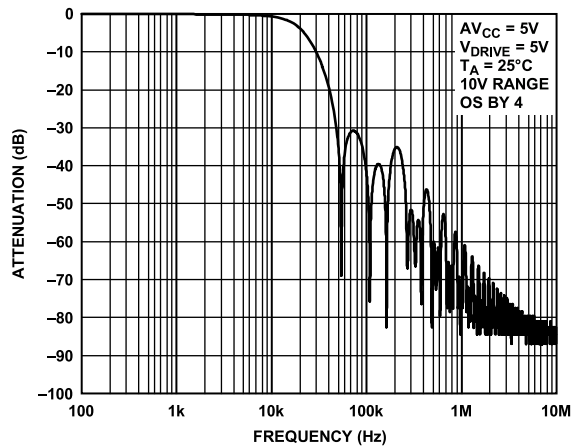
Figure 57. Digital Filter Response for OS 4
