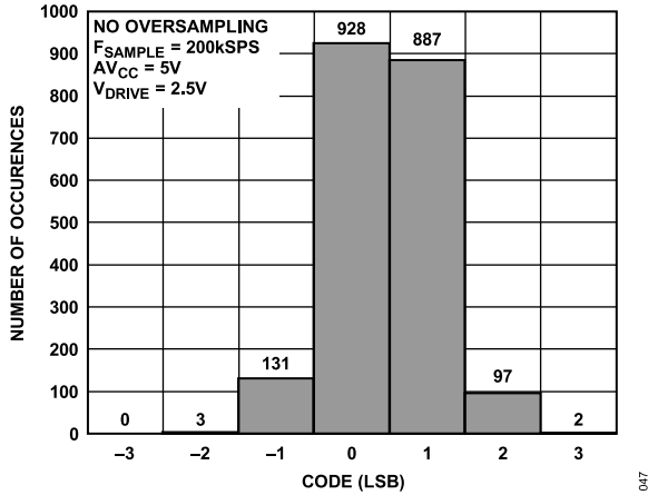
Figure 49. Histogram of Codes—No OS (Six Codes)
