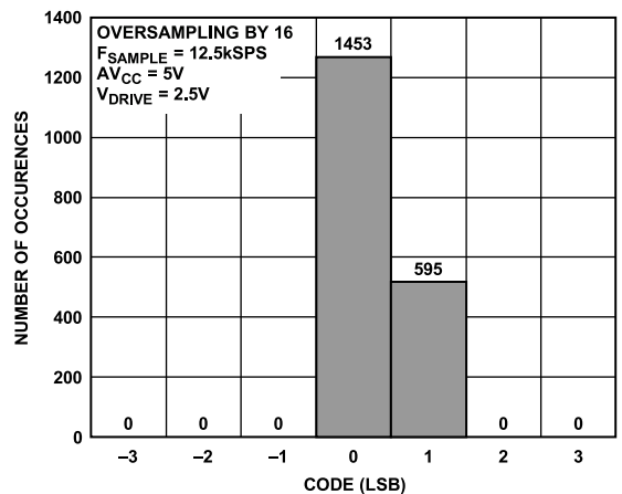
Figure 53. Histogram of Codes—OS x 16 (Two Codes)
