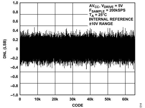
Figure 15. AD7606 Typical DNL, ±10 V Range
