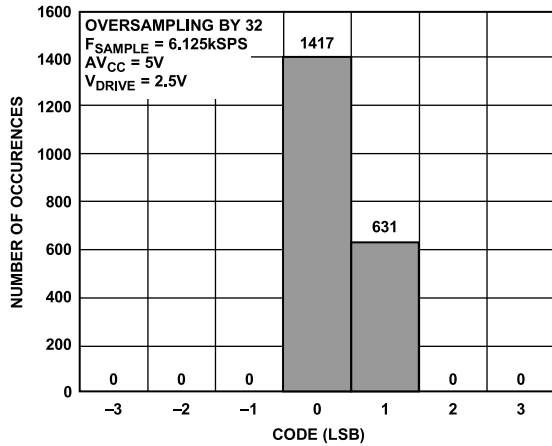
Figure 54. Histogram of Codes—OS x 32 (Two Codes)
