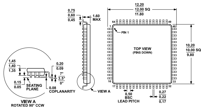
Figure 65. 64-Lead Low Profile Quad Flat Package [LQFP] (ST-64-2) Dimensions shown in millimeters
