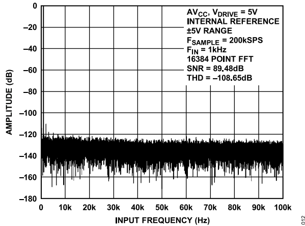
Figure 12. AD7606 FFT Plot, ±5 V Range
