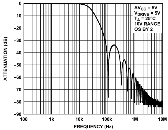
Figure 56. Digital Filter Response for OS 2
