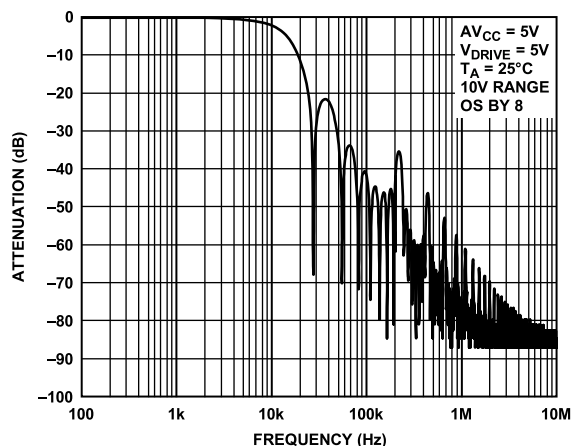
Figure 58. Digital Filter Response for OS 8
