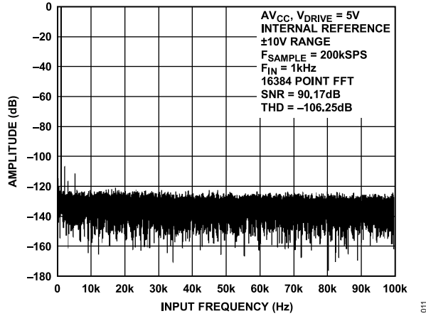
Figure 11. AD7606 FFT, ±10 V Range
