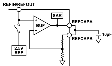
Figure 40. Reference Circuitry
