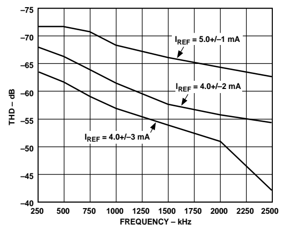
Figure 32. Reference Channel Distortion vs. Frequency
