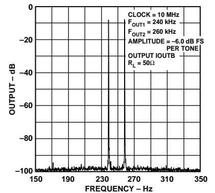
Figure 20. Intermodulation Distortion
