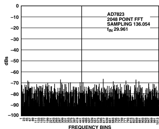
Figure 3. AD7823 SNR
