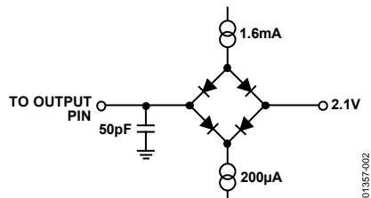
Figure 2. Load Circuit for Access Time and Bus Relinquish Time
