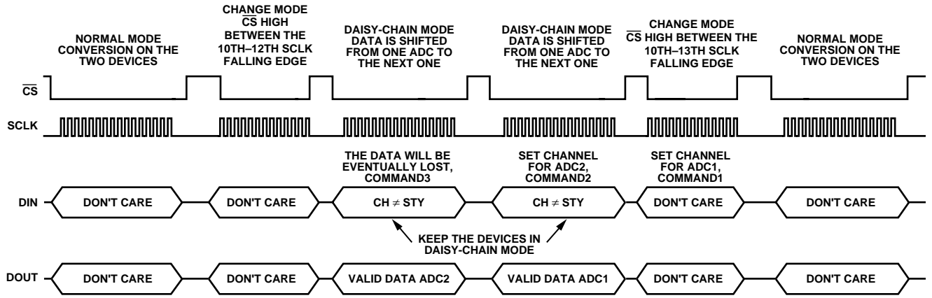
Figure 34. Daisy-Chain Diagrams—1
