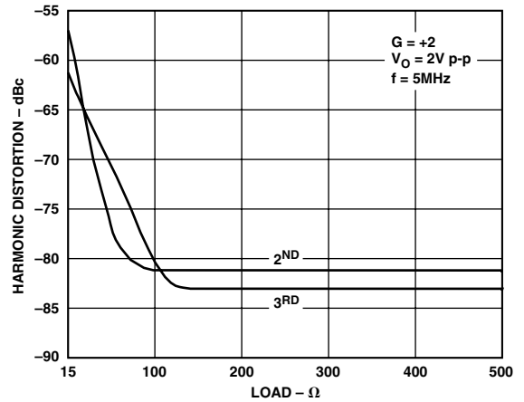
Figure 13. Harmonic Distortion vs. Load
