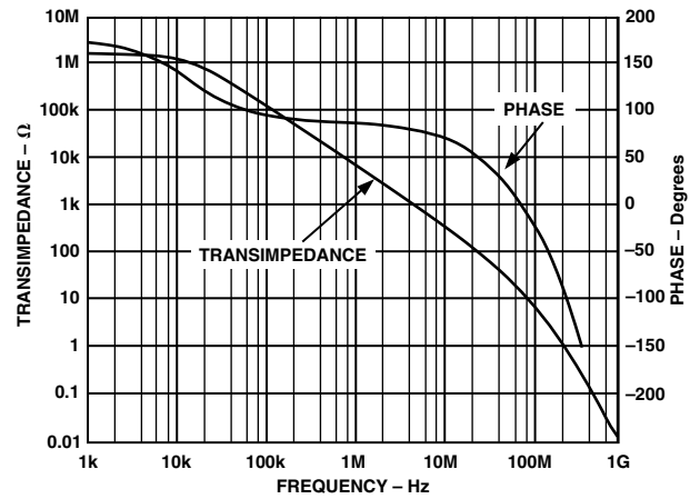
TPC 23. Open Loop Transimpedance and Phase
