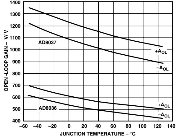
TPC 46. Open-Loop Gain vs. Temperature
