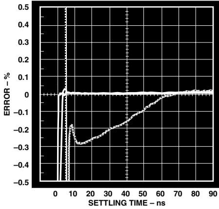
TPC 61. AD8036 Clamp Settling (0.1%), V_H = +1 V , V_L = -1 V , 2x Overdrive
