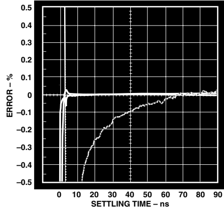
TPC 64. AD8037 Clamp Settling (0.1%), V_H = +0.5 V , V_L = -0.5 V , 2x Overdrive
