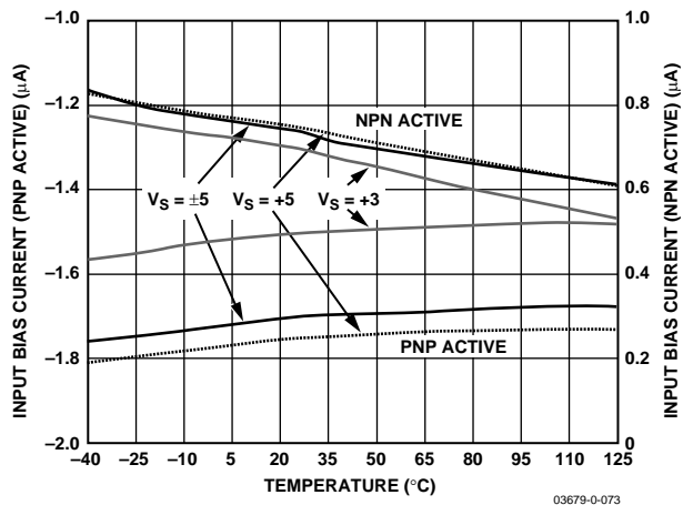
Figure 38. Input Bias Current vs. Temperature
