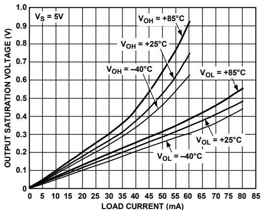
Figure 31. AD8051/AD8052 Output Saturation Voltage vs. Load Current
