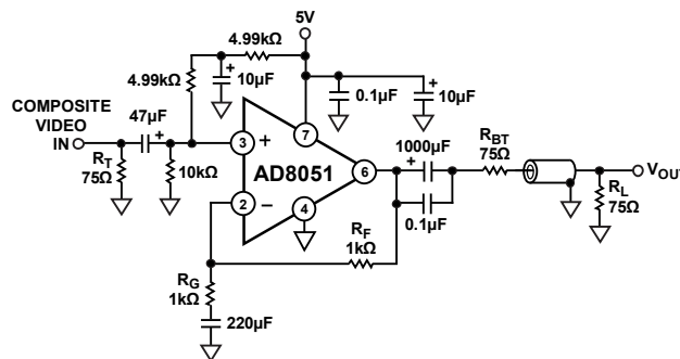
Figure 52. Single-Supply Composite Video Line Driver
