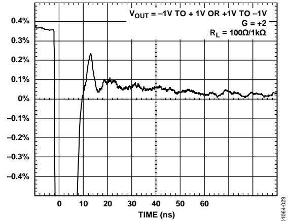
Figure 27. Settling Time
