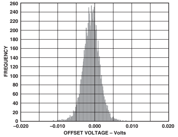
TPC 29. AD8110 Offset Voltage Distribution
