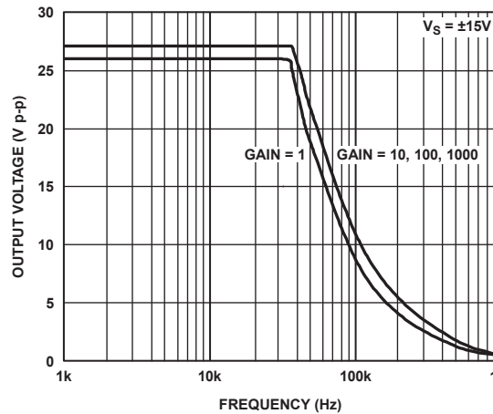
Figure 32. Large Signal Frequency Response
