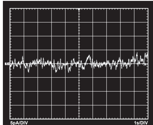
Figure 31. 0.1 Hz to 10 Hz Current Noise
