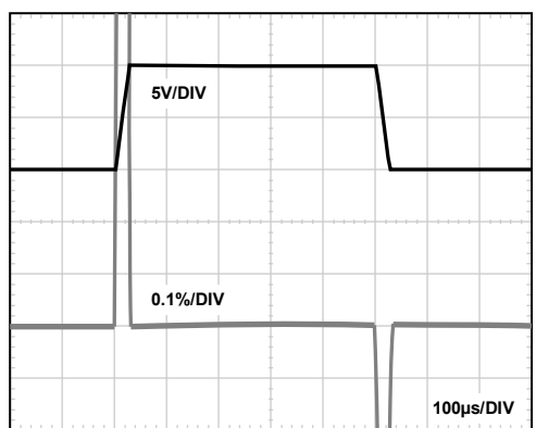
Figure 26. Large Signal Pulse Response, G = 100 , C_L = 100\text{ pF}
