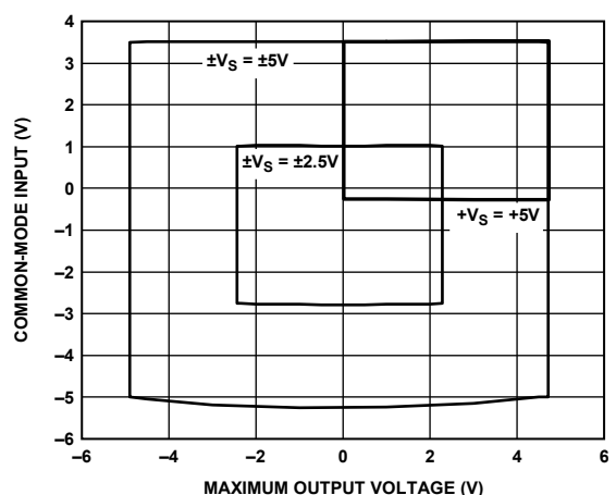
Figure 20. Common-Mode Input vs. Maximum Output Voltage, G = 100 , Small Supplies
