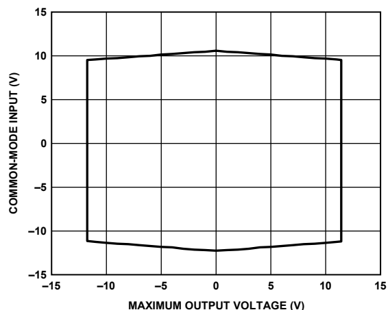
Figure 19. Common-Mode Input vs. Maximum Output Voltage, G = 5 , \pm V_S = \pm 12\text{ V}
