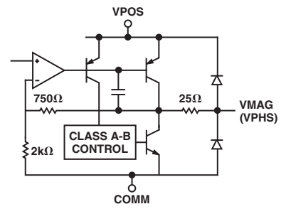
Circuit B
