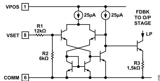
Figure 28. Setpoint Interface Circuitry
