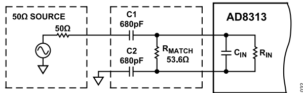
Figure 32. A Simple Broadband Resistive Input Termination
