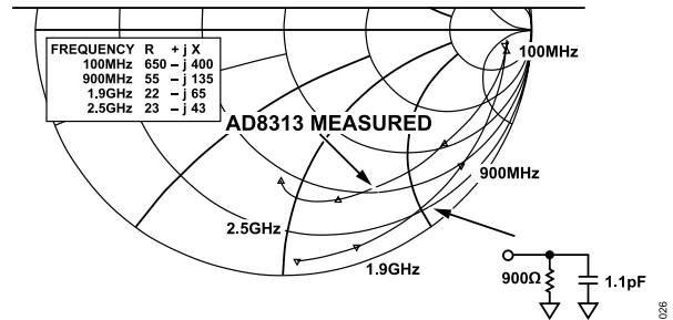
Figure 26. Typical Input Impedance
