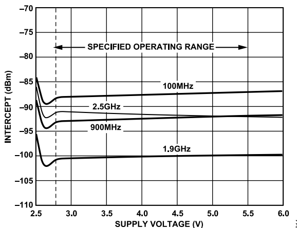
Figure 14. V_{OUT} Intercept vs. Supply Voltage
