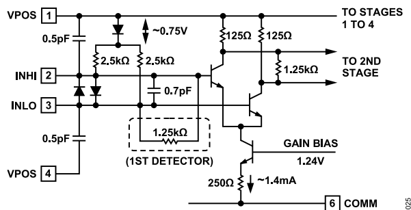
Figure 25. Input Interface Simplified Schematic
