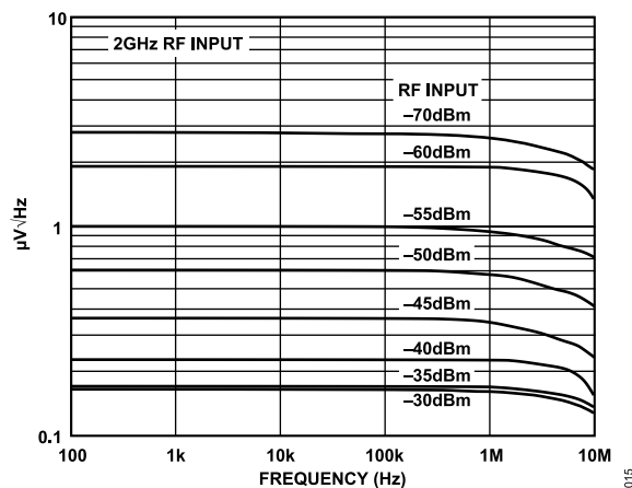
Figure 15. V_{OUT} Noise Spectral Density
