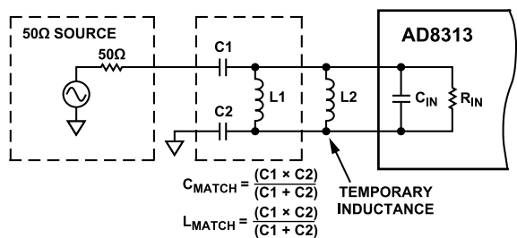
Figure 36. Input Matching Example
