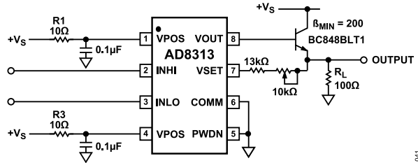
Figure 41. Output Current Drive Boost Connection
