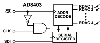
Figure 49. Equivalent Input Control Logic
