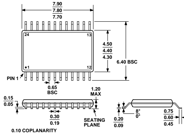
COMPLIANT TO JEDEC STANDARDS MO-153-AD Figure 64. 24-Lead Thin Shrink Small Outline Package [TSSOP] (RU-24) Dimensions shown in millimeters
