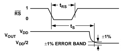
Figure 5. Reset Timing Diagram
