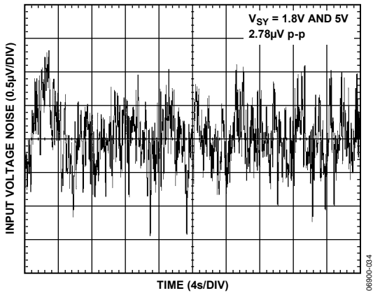
Figure 39. Input Voltage Noise 0.1 Hz to 10 Hz
