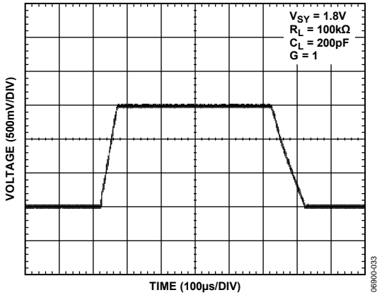
Figure 37. Large-Signal Transient Response
