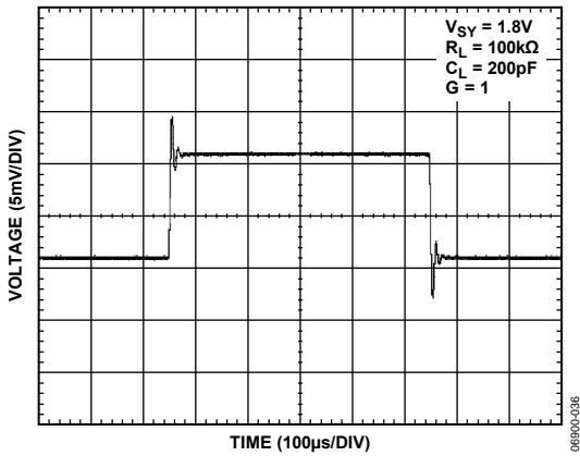
Figure 38. Small-Signal Transient Response
