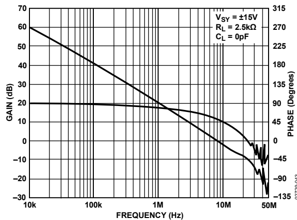
Figure 47. Frequency Response of the AD8510/AD8512/AD8513
