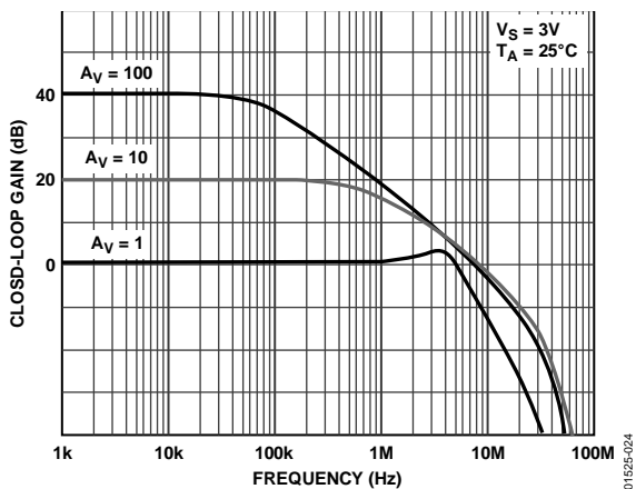
Figure 24. Closed-Loop Gain vs. Frequency
