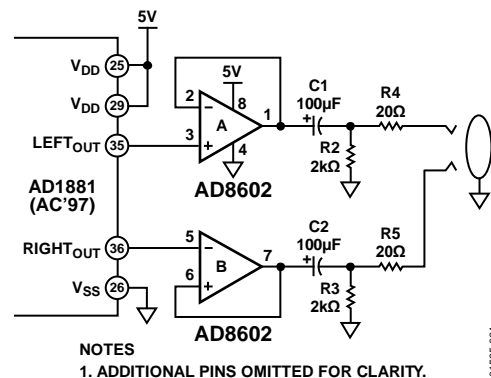
Figure 61. A PC100-Compliant Line Output Amplifier
