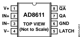
Figure 4. 8-Lead Narrow Body SOIC Pin Configuration
