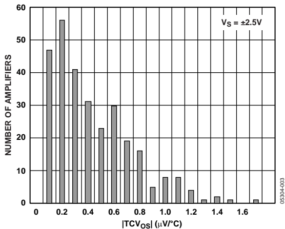
Figure 5. |TCV_{0s}| Distribution
