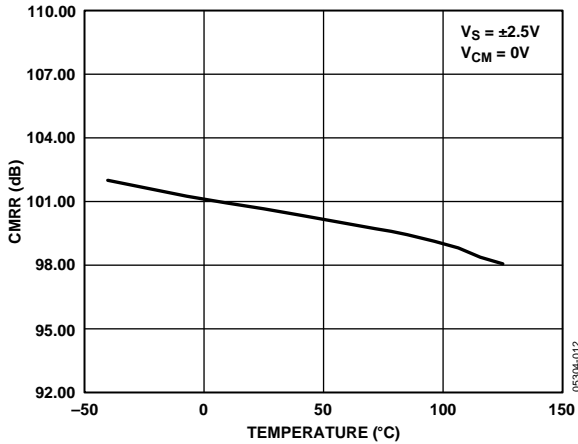
Figure 15. Large Signal CMRR vs. Temperature
