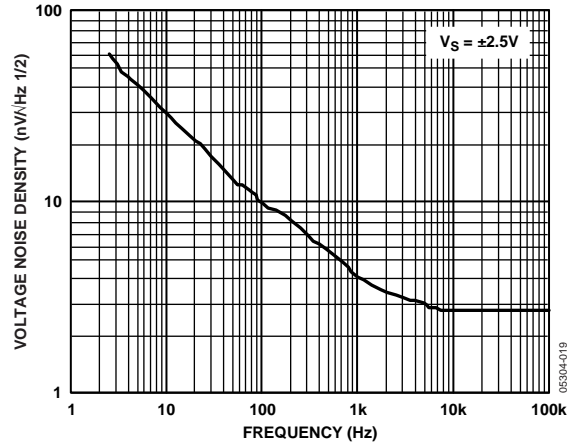
Figure 18. Voltage Noise Density vs. Frequency
