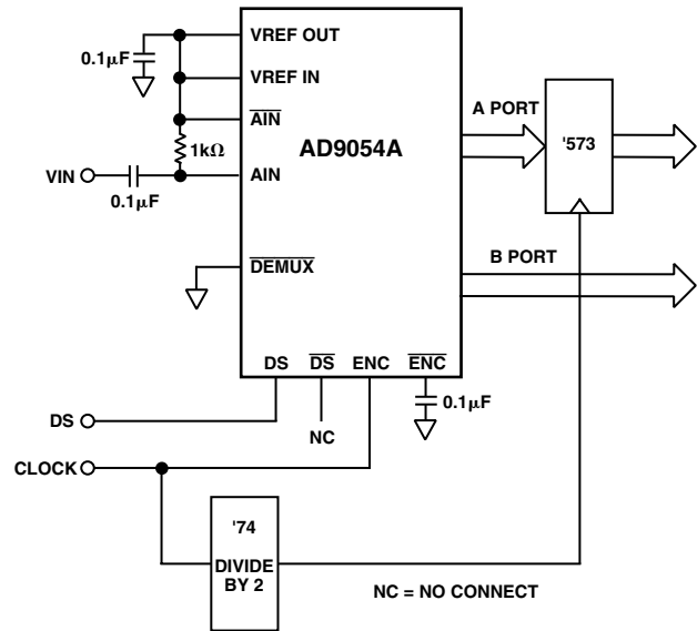
Figure 11. Dual Port Mode—Aligned Output Data
