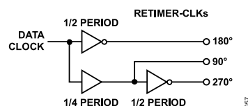
Figure 95. RETIMER-CLK Phases
