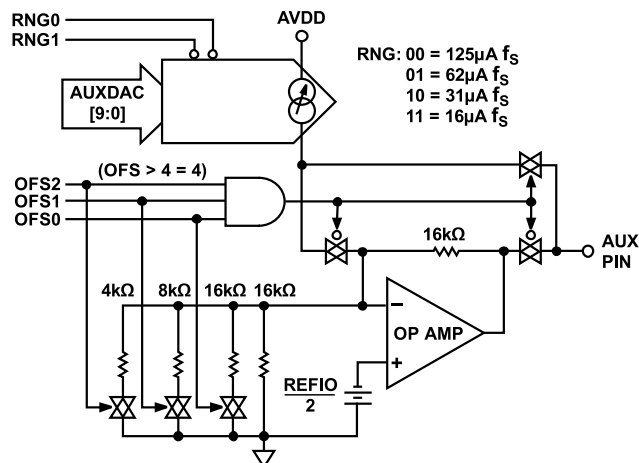
Figure 106. AUXDAC Simplified Circuit Diagram
