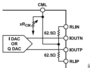
Figure 101. Simplified Internal Load Options
