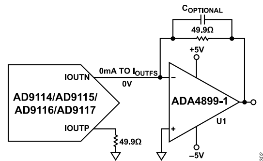
Figure 104. Unipolar Buffered Voltage Output
