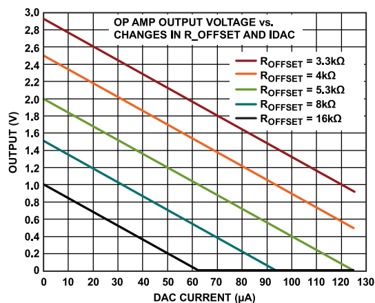
Figure 107. AUXDAC Op Amp Output vs. Current, AVDD = 3.3 V No Load, AUXDAC 0x1FF to 0x000
