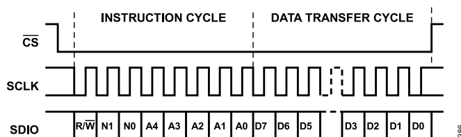
Figure 86. Serial Register Interface Timing, MSB First Read
